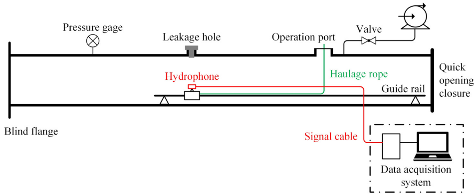
Fig. 2. Experimental apparatus for testing leak-induced sound characteristics.
